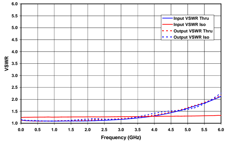
Figure 4. Input and Output Return Loss vs. Frequency
