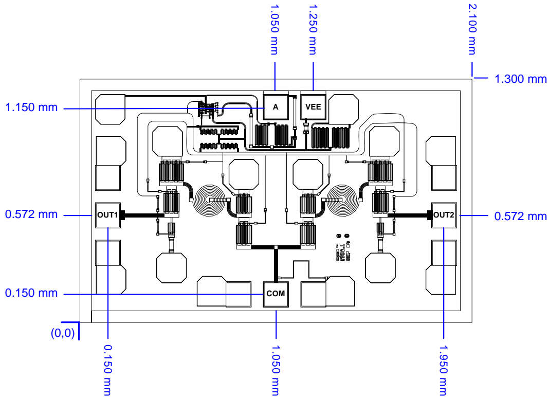
Figure 5. Die Layout
